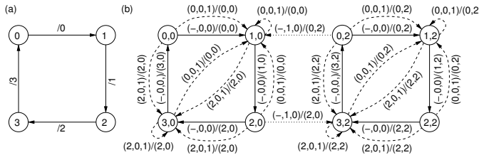
Figure 2: (a) FSM of a modulo-4-counter. (b) Corresponding CFMSM for S_c = \{0, 2\} , i.e., only in states 0 and 2 saving of a checkpoint is permitted. The state space is given by the actual state and the last saved checkpoint.
