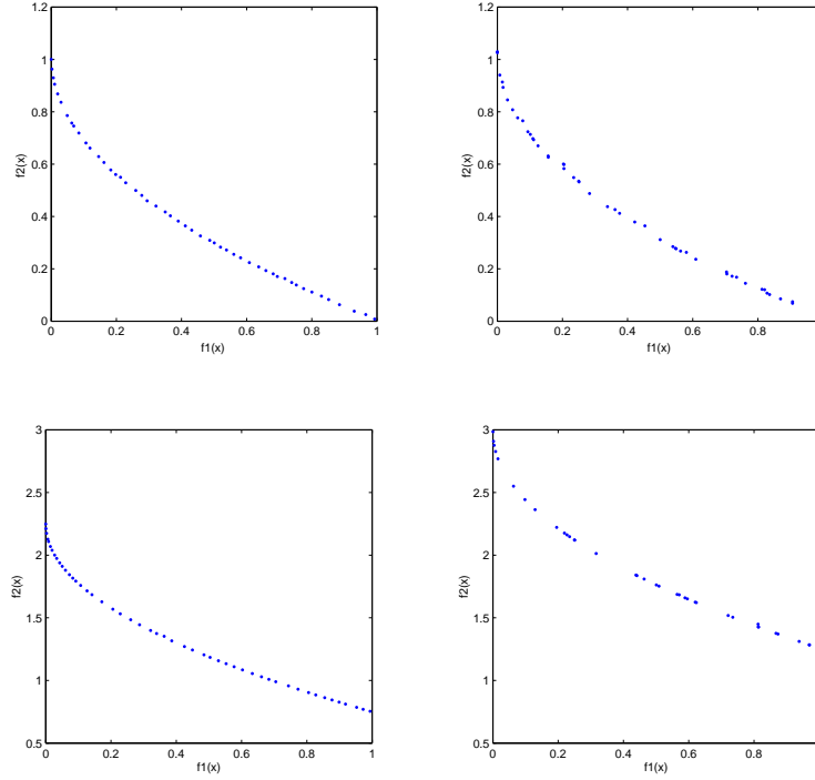
Fig. 7. Continuous Pareto-optimal fronts. Solutions of ZDT1 (first row) and ZDT4 (second row) in the objective space. The left and right columns illustrate the results of the methods A and B, respectively.
