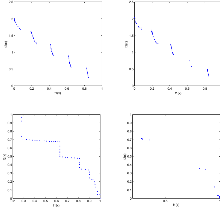
Fig. 8. Continuous and disconnected Pareto-optimal fronts. Solutions of ZDT3 (first row) and ZDT6 (second row) in the objective space. The left and right columns illustrate the results of the methods A and B, respectively.
