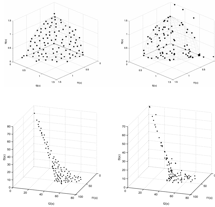
Fig. 9. Continuous Pareto-optimal fronts. Solutions of GSP3 (first row) and CP3 (second row) in the objective space. The left and right columns illustrate the results of the methods A and B, respectively.
